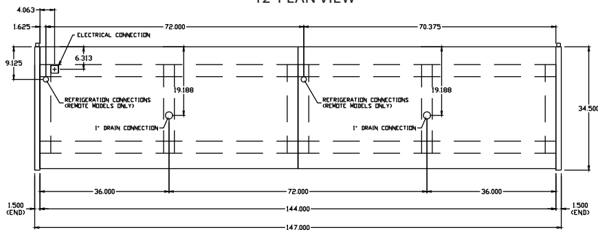
12' PLAN VIEW
