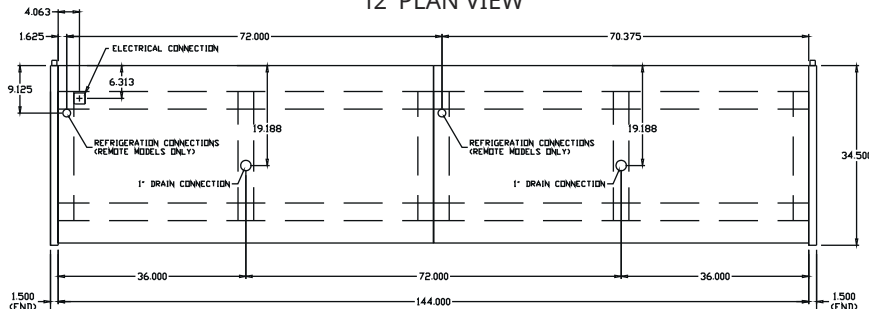
12' PLAN VIEW
