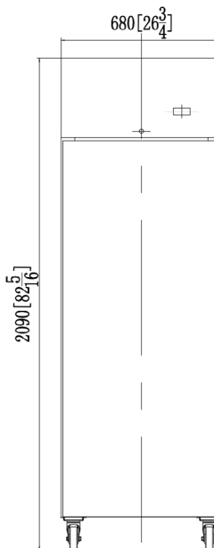
FRONT VIEW
