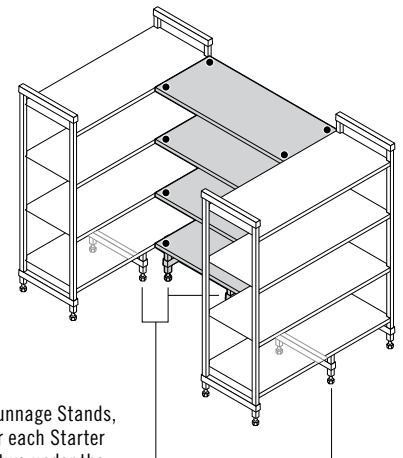
• = Corner Connectors
