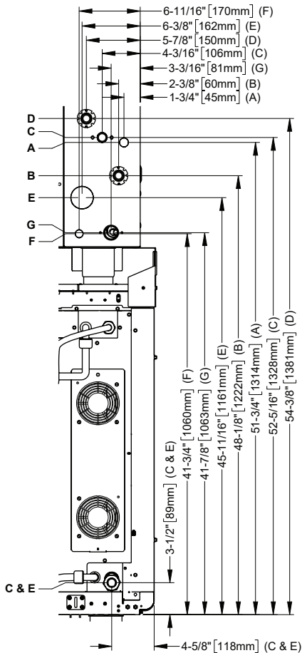
DETAIL X
