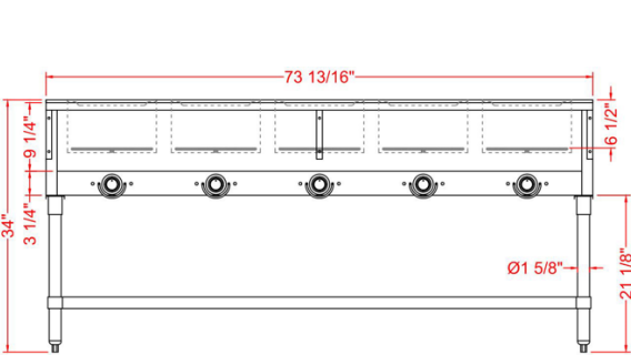
FRONT
