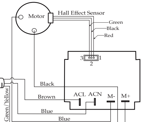
Wiring Diagram
