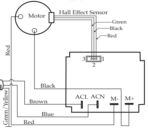
Wiring Diagram (on units after 11/1/2017)
