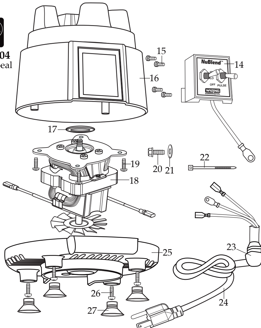
503408 Blending Assembly
