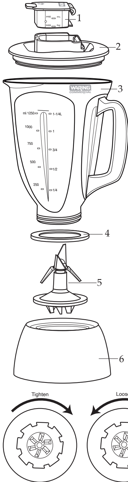
503408 Blending Assembly
