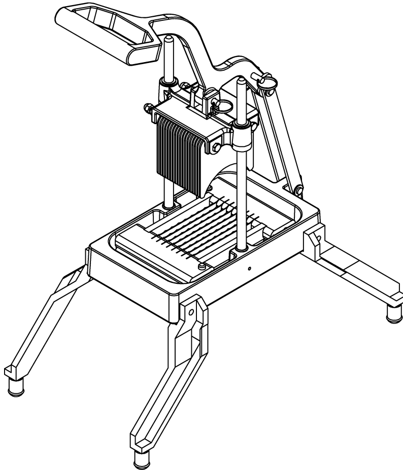
56750-( ) CARTRIDGE ONION SLICER
