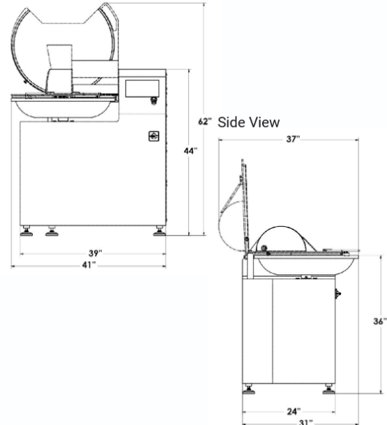
46216 Front View
