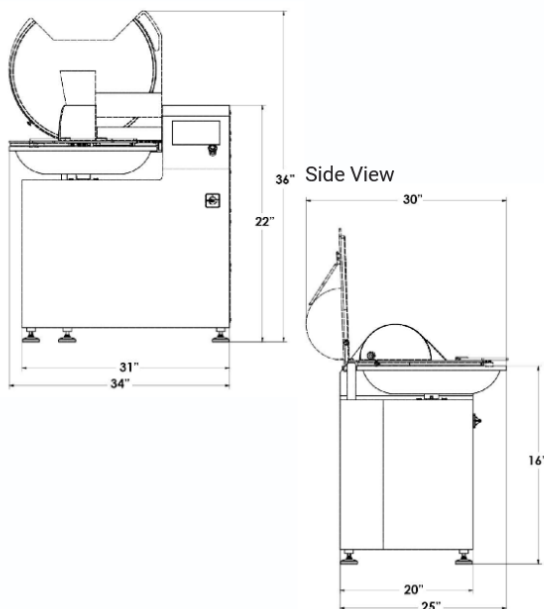
46215 Front View
